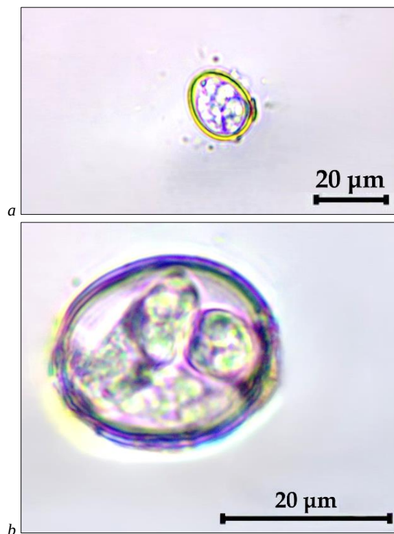
Fig. 1. Oocysts of Eimeria tenella in control test cultures: a, b – sporulated
