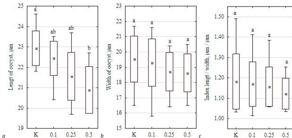
Fig. 2. Metric parameters of Eimeria tenella oocysts in test cultures when using the disinfectant "Virosan" in different concentrations with an exposure of 150 min: a – length of oocyst ( \mu\text{m} ), b – width of oocyst ( \mu\text{m} ), c – length/width index ( \mu\text{m}/\mu\text{m} ); K – control; the small square in the center corresponds to the median, the lower and upper borders of the large rectangular correspond to the first and the third quartiles, respectively, vertical line segments, directed up and down from the rectangular, correspond to minimum and maximum values ( n = 14 ); different letters in the figure indicate significant ( P < 0.05 ) differences between groups according to Tukey test results
