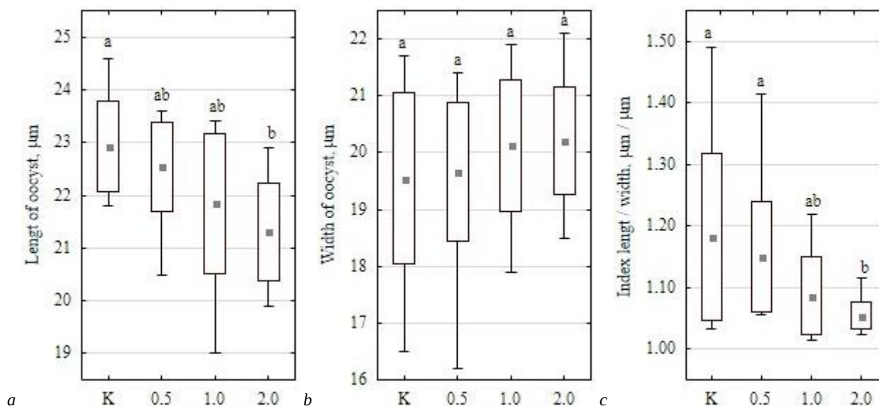
Fig. 3. Metric parameters of Eimeria tenella oocysts in test cultures when using the disinfectant "Yoderyn" in different concentrations with an exposure of 150 min: for notes, see Fig. 2
